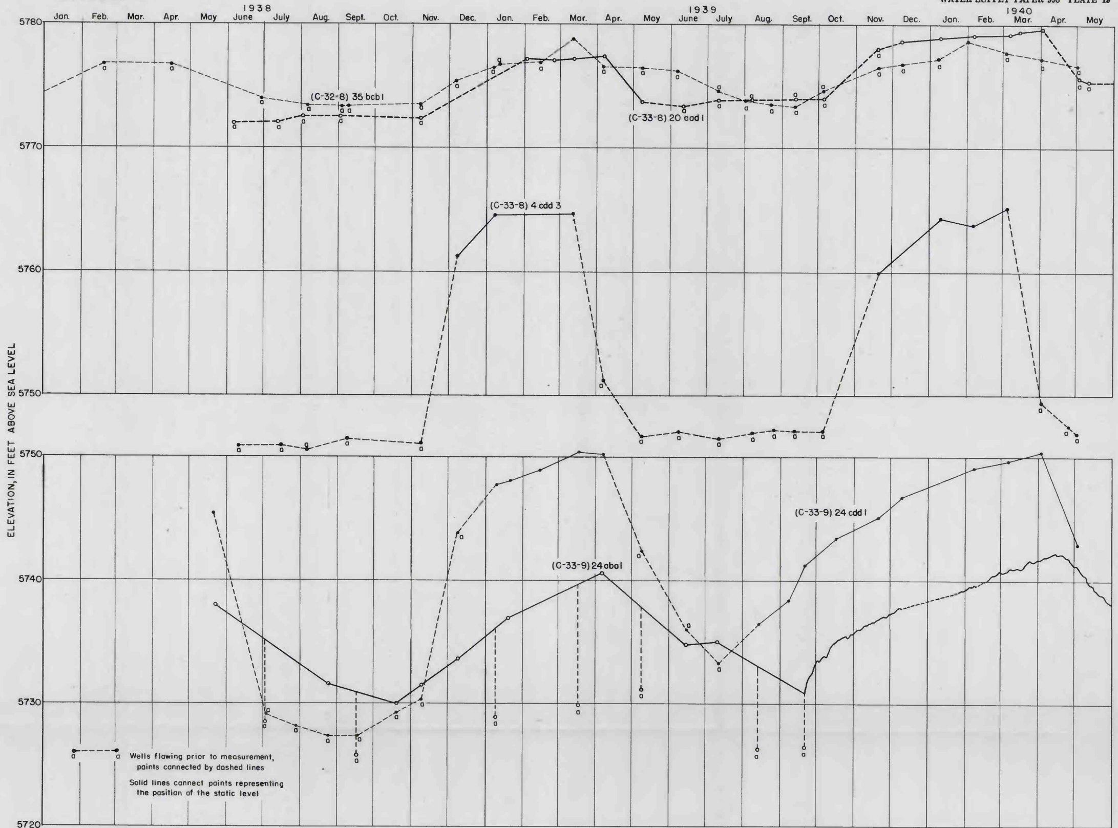
HYDROGRAPHS OF FIVE WELLS IN WHICH THE SEASONAL FLUCTUATIONS OF STATIC LEVEL ARE CAUSED CHIEFLY BY FLOW FROM ARTESIAN WELLS
