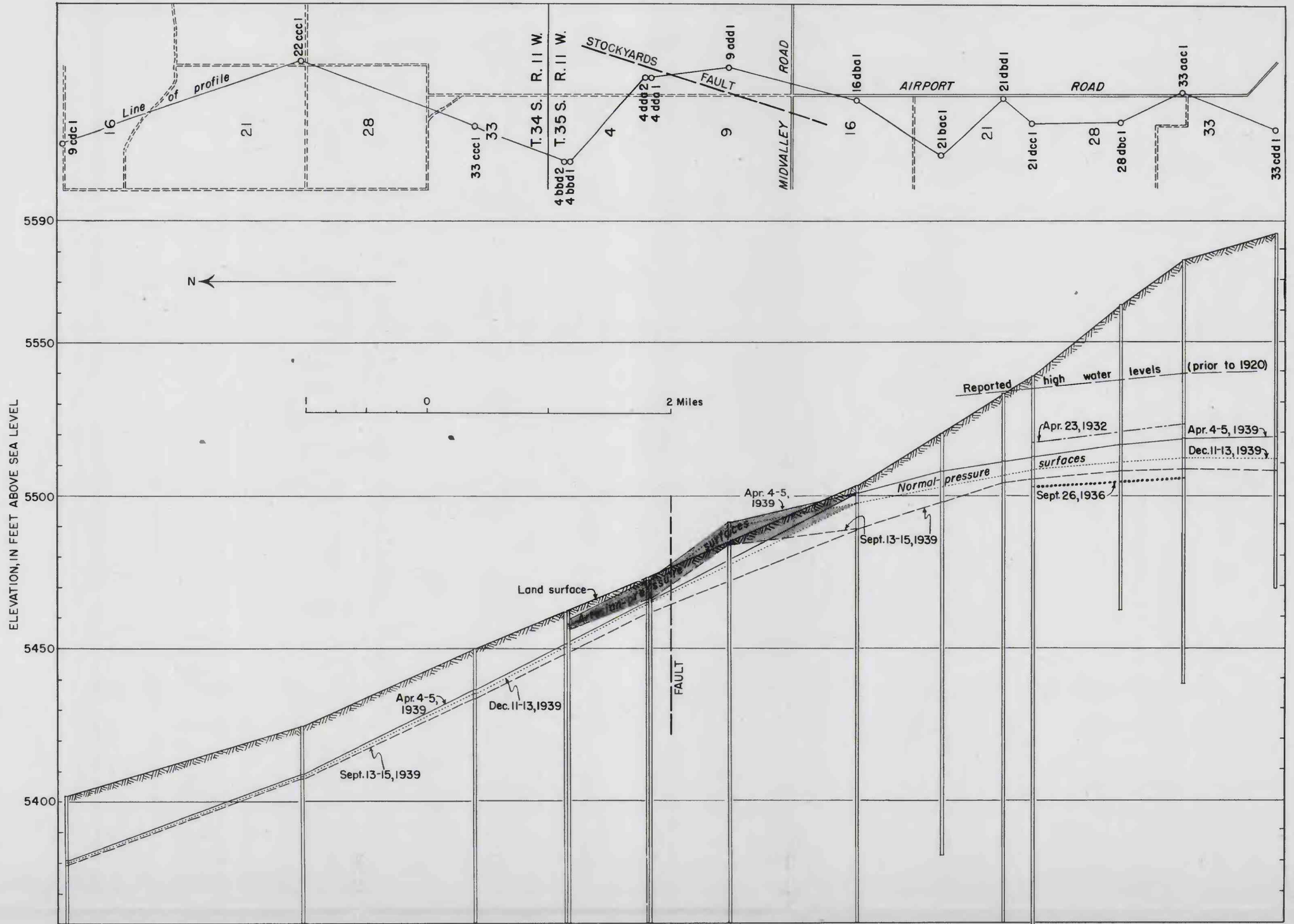
NORTH-SOUTH PROFILE APPROXIMATELY THROUGH THE CENTER OF T.P.S. 34 AND 35 S., R. 11 W., SHOWING POSITIONS OF THE WATER SURFACE DURING 1932, 1936, AND 1939
