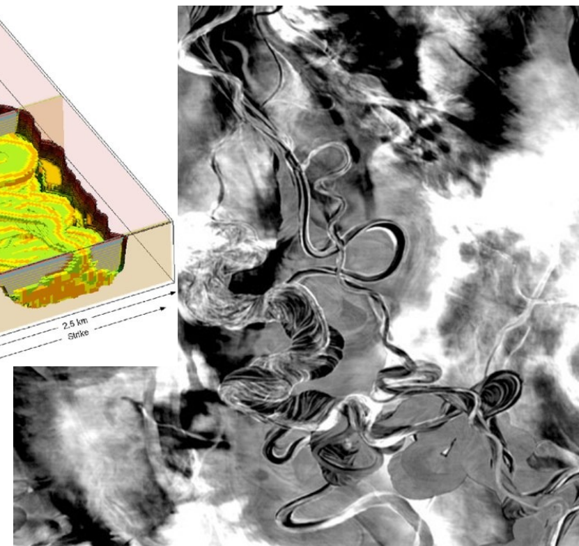
3-D seismic horizontal slice showing fluvial channels
