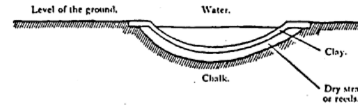
Figure 40 ~ Dew Pond (Oxtedde Bottom, Sussex):
