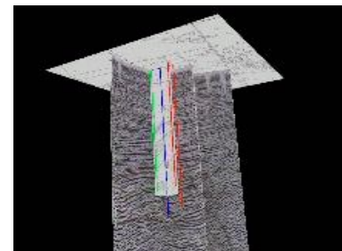
Spatial Correlation of Base Map, 2D Seismic and Well Data
