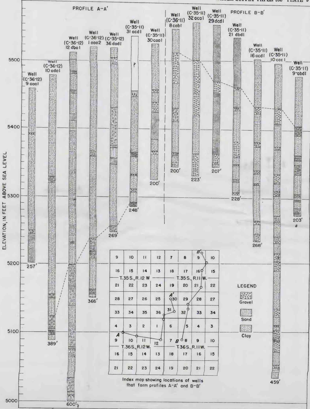
WELL SECTIONS BASED ON DRILLERS' LOGS FOR SEVERAL WELLS THAT FORM TWO CROOKED BUT ROUGHLY PARALLEL PROFILES ALONG THE COAL CREEK FAN IN CEDAR CITY VALLEY
